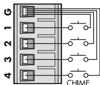
⑨ Connection of the chime pushbutton
